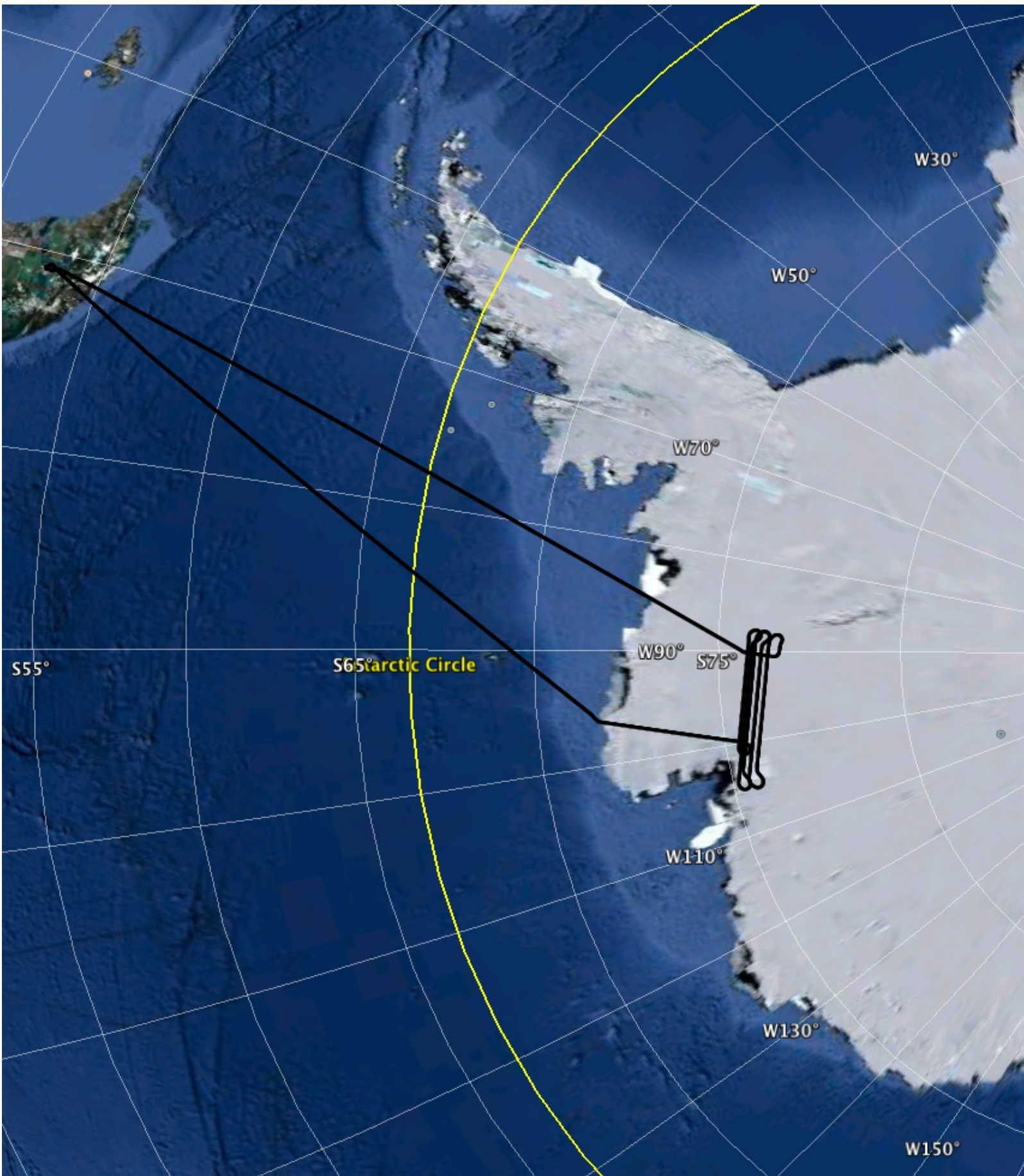
Pine Island Glacier 2
