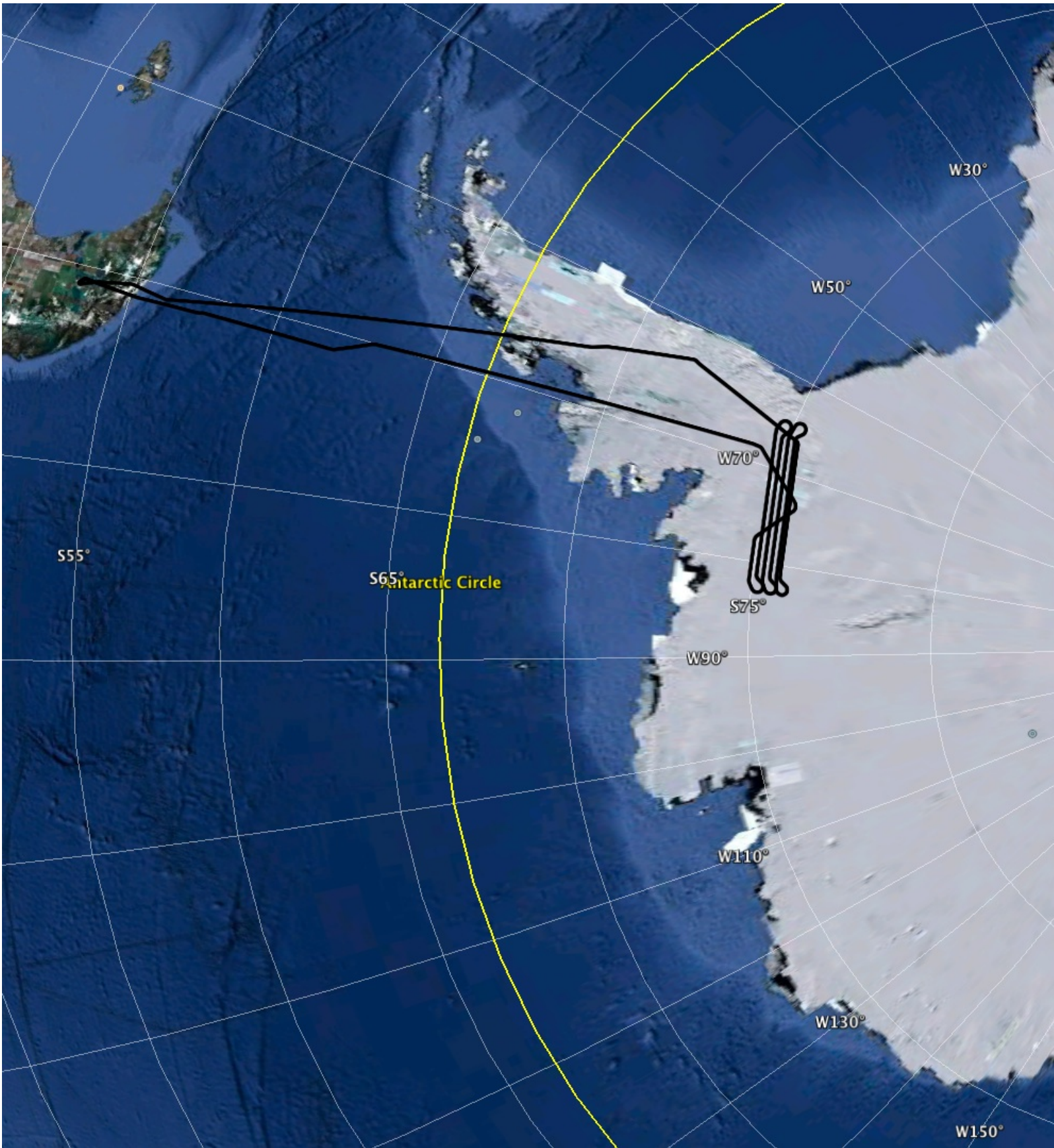
Drewry Ice Stream
